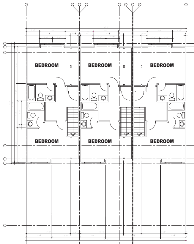
TOWNHOME BUILDING TYPE 1, 3-PLEX UPPER LEVEL (3) 2B, 2-1/2BA UNITS
