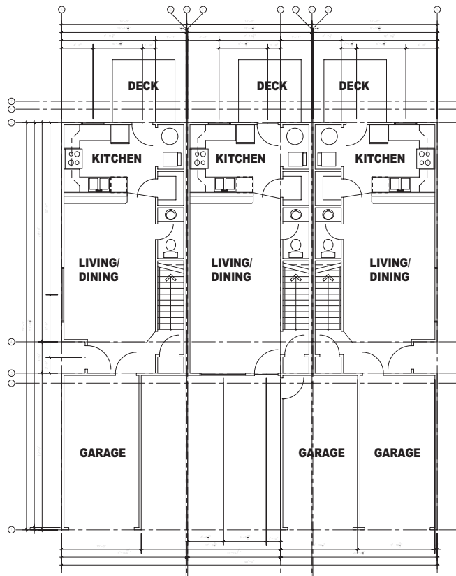
TOWNHOME BUILDING TYPE 1, 3-PLEX LOWER LEVEL (3) 2B, 2-1/2BA UNITS
