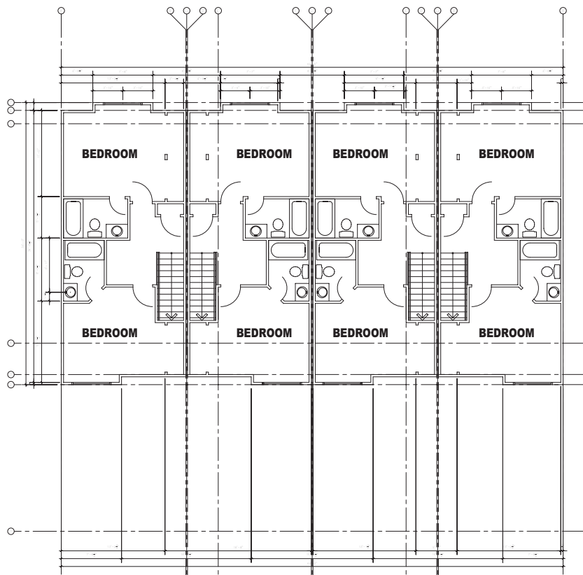
TOWNHOME BUILDING TYPE 1, 4-PLEX UPPER LEVEL (4) 2B, 2-1/2BA UNITS
