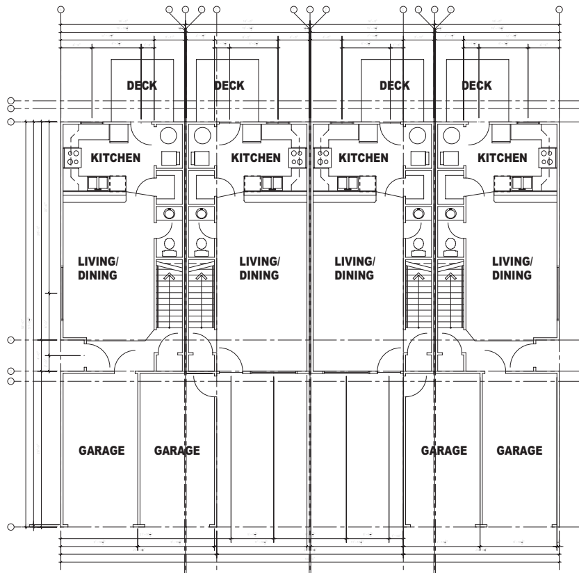
TOWNHOME BUILDING TYPE 1, 4-PLEX LOWER LEVEL (4) 2B, 2-1/2BA UNITS
