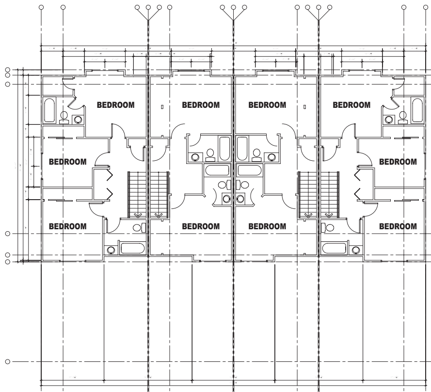
TOWNHOME BUILDING TYPE 2, 4-PLEX UPPER LEVEL (2) 2B, 2-1/2BA UNITS (2) 3B, 2-1/2BA UNITS
