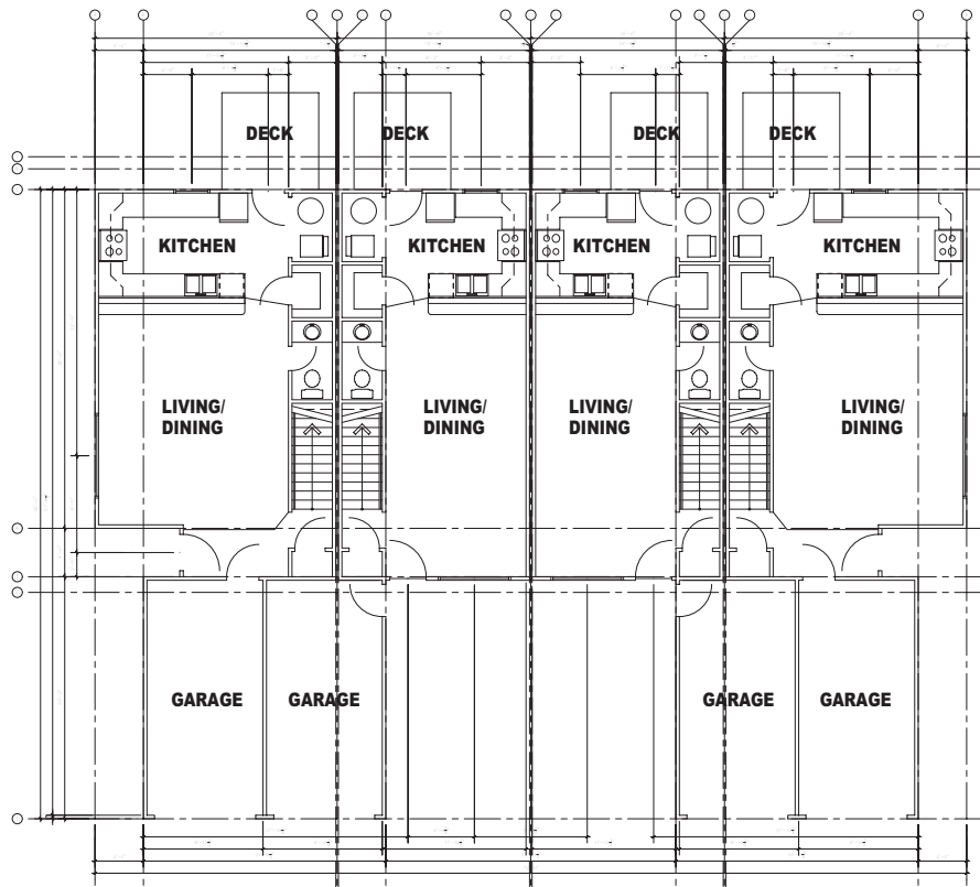
TOWNHOME BUILDING TYPE 2, 4-PLEX LOWER LEVEL (2) 2B, 2-1/2BA UNITS (2) 3B, 2-1/2BA UNITS
