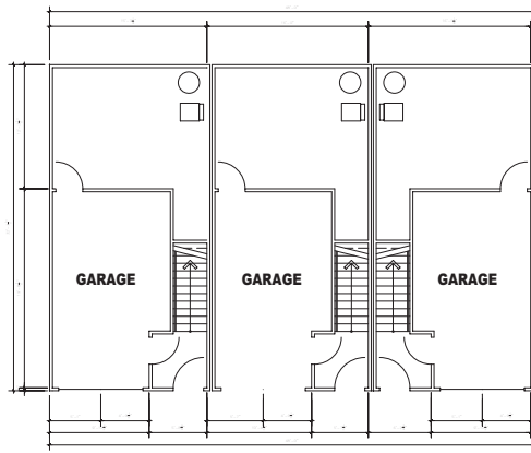
TOWNHOME BUILDING TYPE 3, 3-PLEX LOWER LEVEL (1) 2B, 2-1/2BA UNITS (2) 3B, 2-1/2BA UNITS
