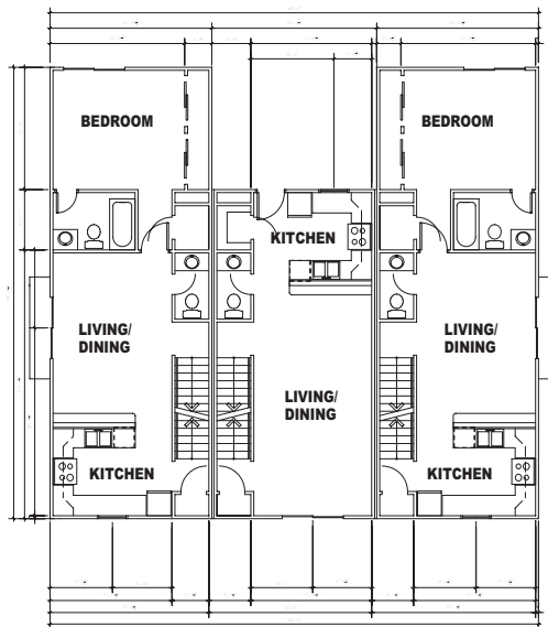
TOWNHOME BUILDING TYPE 3, 3-PLEX MIDDLE LEVEL (1) 2B, 2-1/2BA UNITS (2) 3B, 2-1/2BA UNITS
