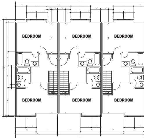
TOWNHOME BUILDING TYPE 3, 3-PLEX UPPER LEVEL (1) 2B, 2-1/2BA UNITS (2) 3B, 2-1/2BA UNITS
