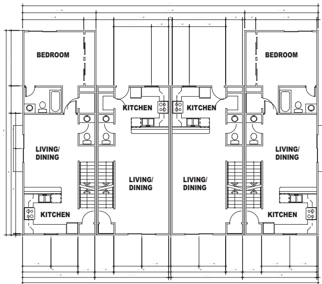
TOWNHOME BUILDING TYPE 3, 4-PLEX MIDDLE LEVEL (2) 2B, 2-1/2BA UNITS (2) 3B, 2-1/2BA UNITS
